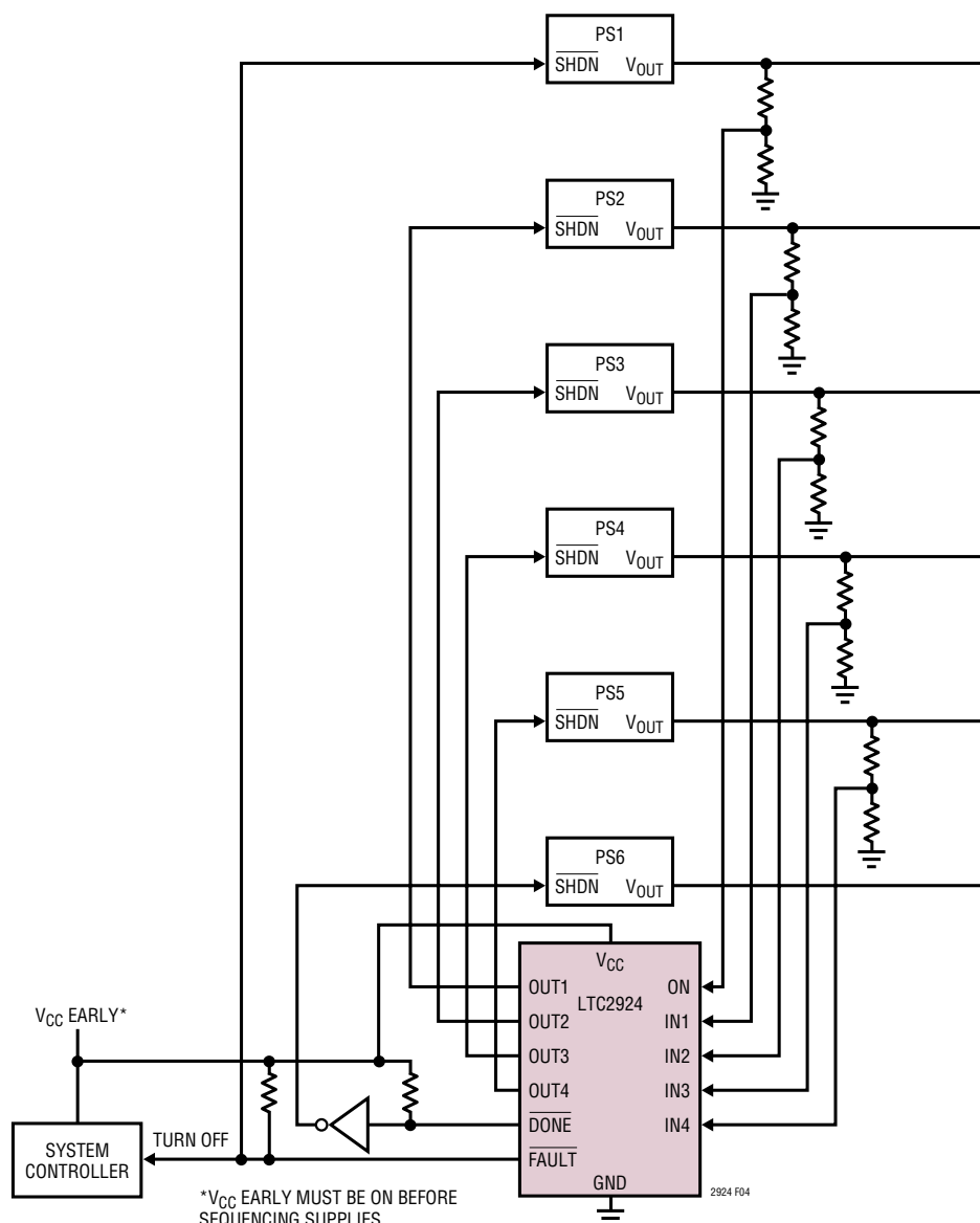
Figure 4. 6-Power Supply Sequencer Block Diagram
