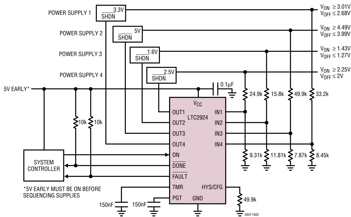
Power On Sequence Timer Delay Longer than Power Off Sequence Timer Delay
